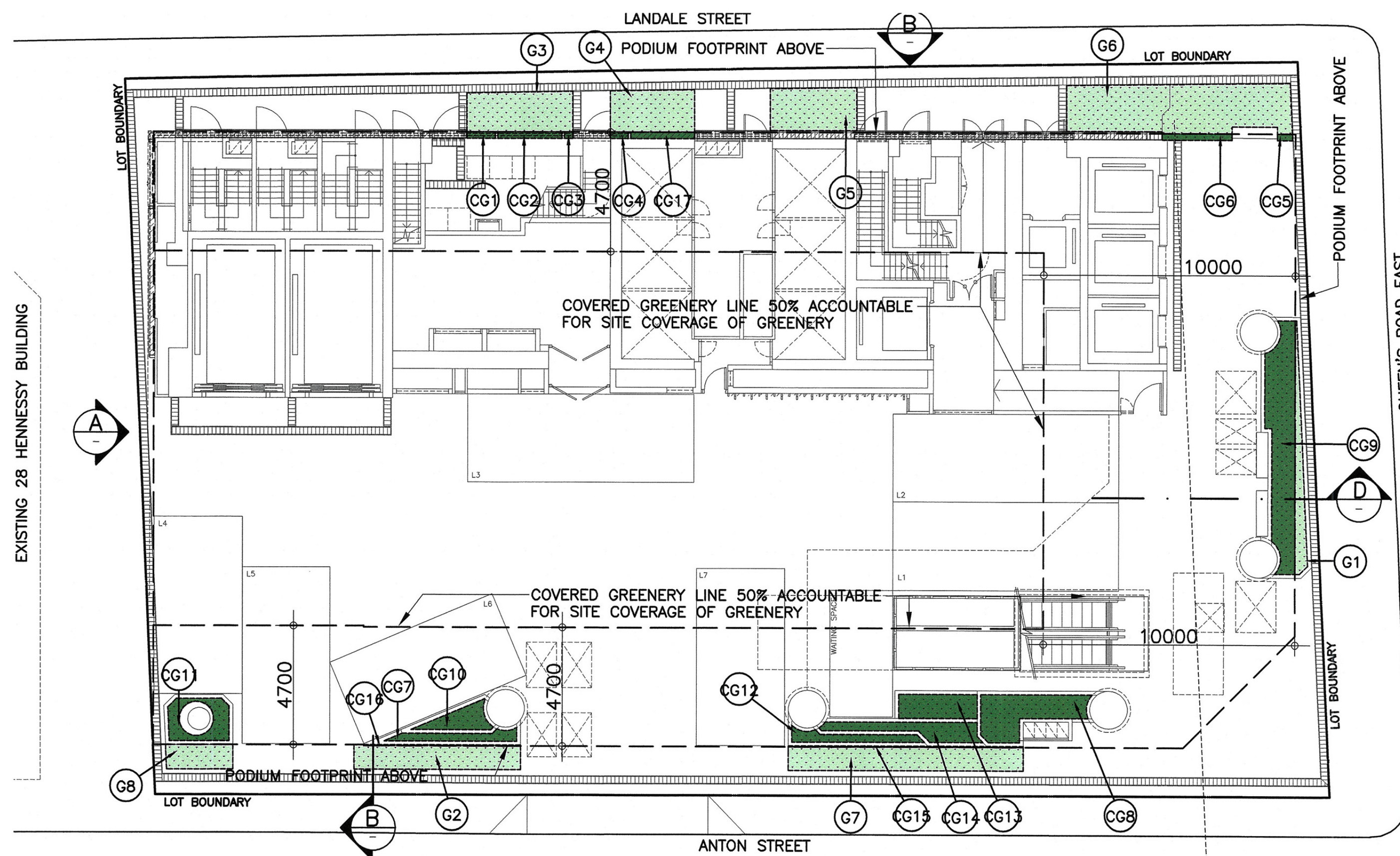
SITE COVERAGE OF GREENERY DIAGRAM G/F ALL AREAS AT G/F ARE ACCESSIBLE TO THE PUBLIC.
